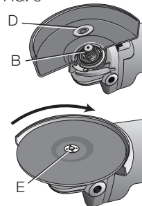
1/4" WHEELS (6.35 mm)
